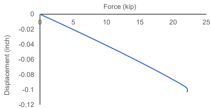
Figure 37 Force-displacement curve at ambient temperature.
