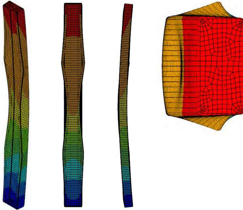
Figure 44 Failure mode under ASTM E119 fire.
