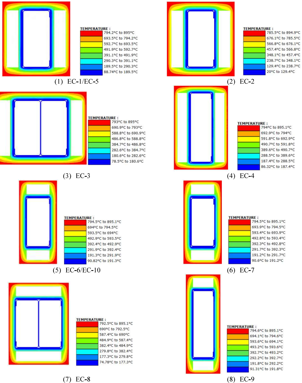
Figure 30 Temperature distribution of each column at 60 minutes under OZone fire_ Warehouse area _50%.
