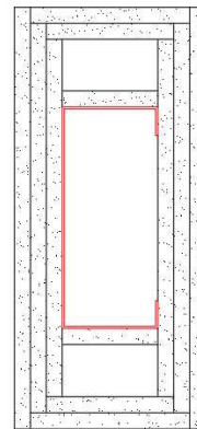
(2) 2-hour rated assembly with 3 layers of ½'' Type C gypsum
